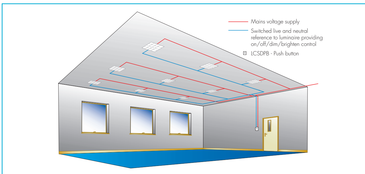
Typical Manual Dimming System wiring schematic
